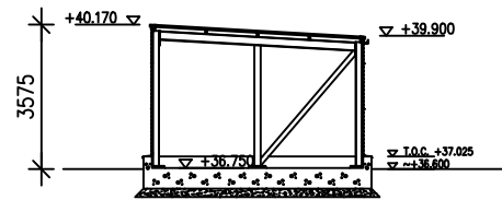
SECTION B
