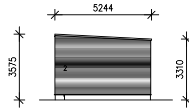
WEST ELEVATION
