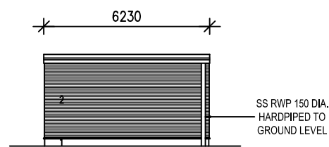
SOUTH ELEVATION
